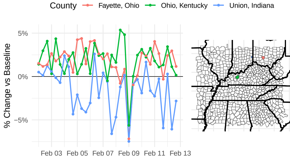
Figure 5: The figure shows that “average change” includes both large increases and large decreases when counties are selected using median absolute percent change in population. The three counties with average change have more variation in population change with both positive and negative changes.
