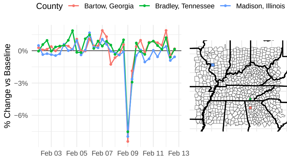
Figure 6: The figure shows that “lowest change” includes one large decrease when counties are selected using lowest absolute percent change in population. The three counties with the lowest change have a notable drop into extreme negative population change on February 9th.
